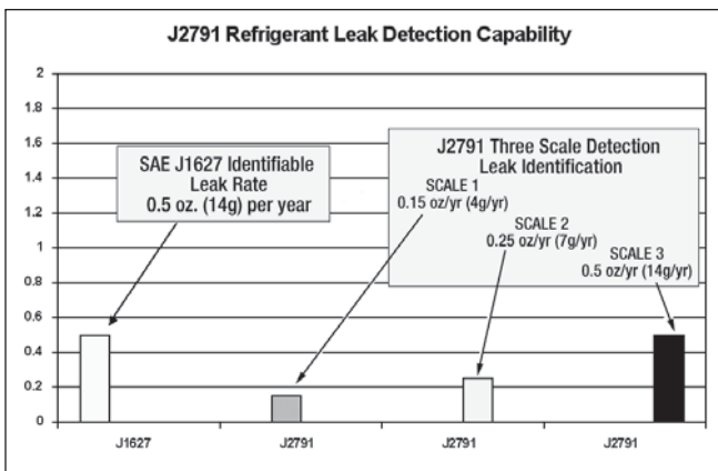
Chart B: This chart compares the effectiveness of SAE J1627 and J2791 electronic leak detectors.
